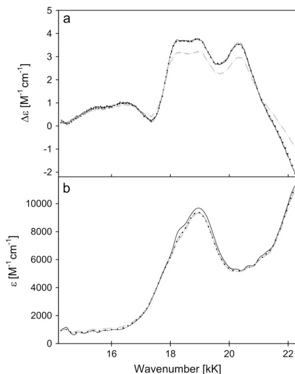
FIGURE 7 ECD ( a ) and absorption ( b ) spectra of the Q -band spectrum of ferri-horse heart (—), bovine (---), chicken (···), and yeast (- · - ·) cytochromes c .
