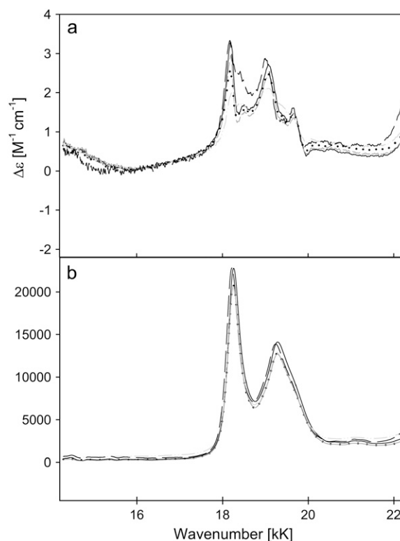
FIGURE 9 ECD ( a ) and absorption ( b ) spectra of the Q -band region of ferri-horse heart (—), bovine (---), chicken (···), and yeast (- · - ·), and Y67F mutant (—) cytochromes c .
