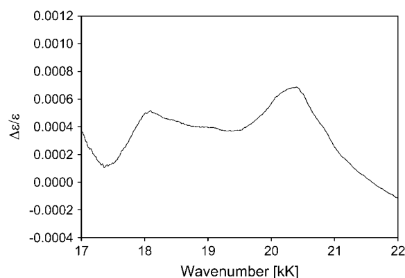
FIGURE 8 Kuhn anisotropy Q -band spectrum of horse heart ferri-cytochrome c .
